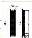
9 Cups Cake Pan
